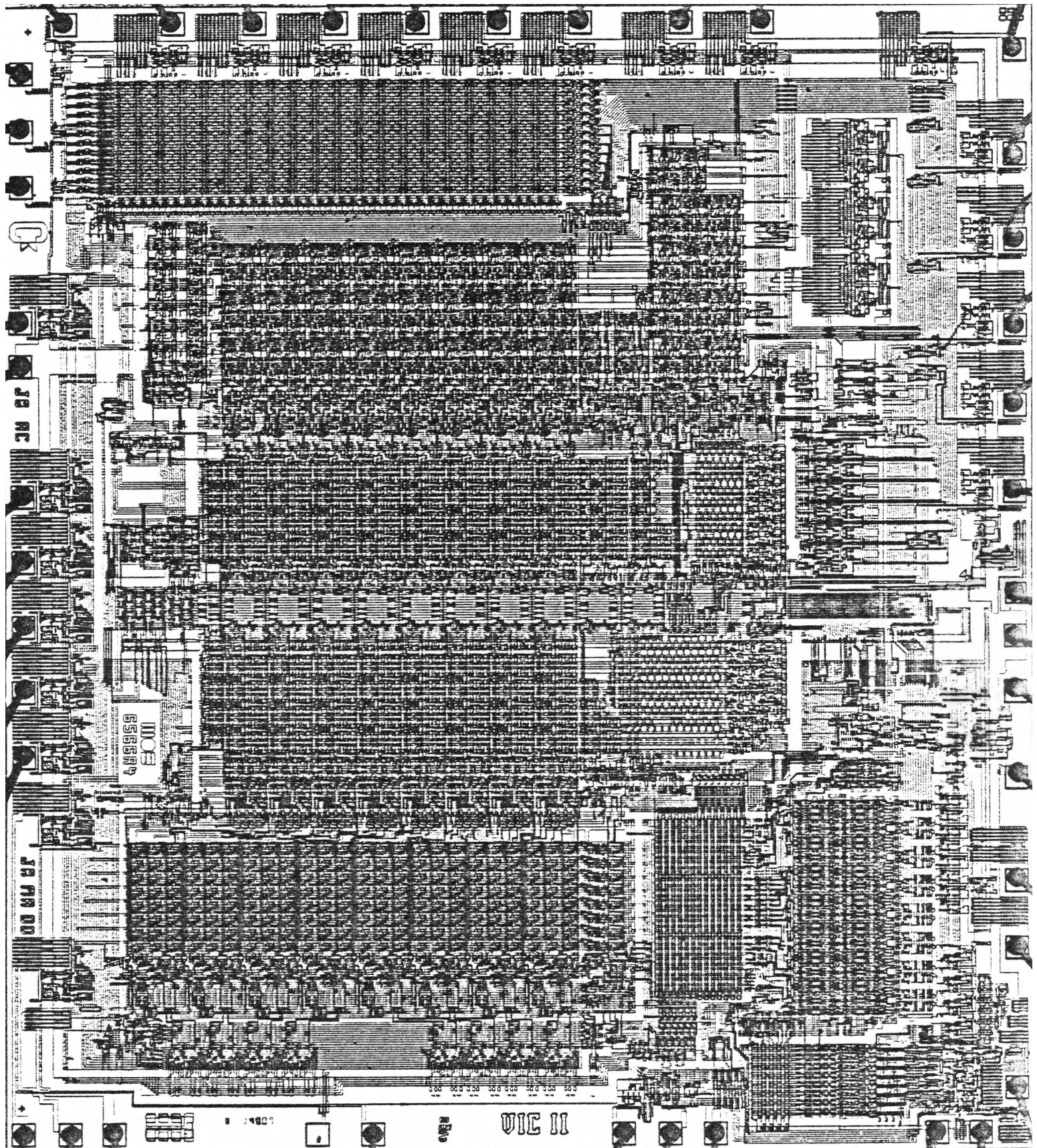
MOS Technology MOS6566 (Implemented on Commodore MAX; 4μ process, 5.9mm square)
