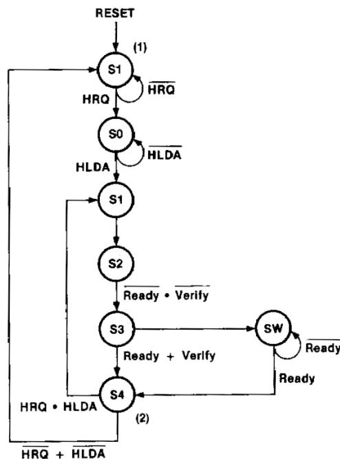
Figure 1. DMA Operation State Diagram
