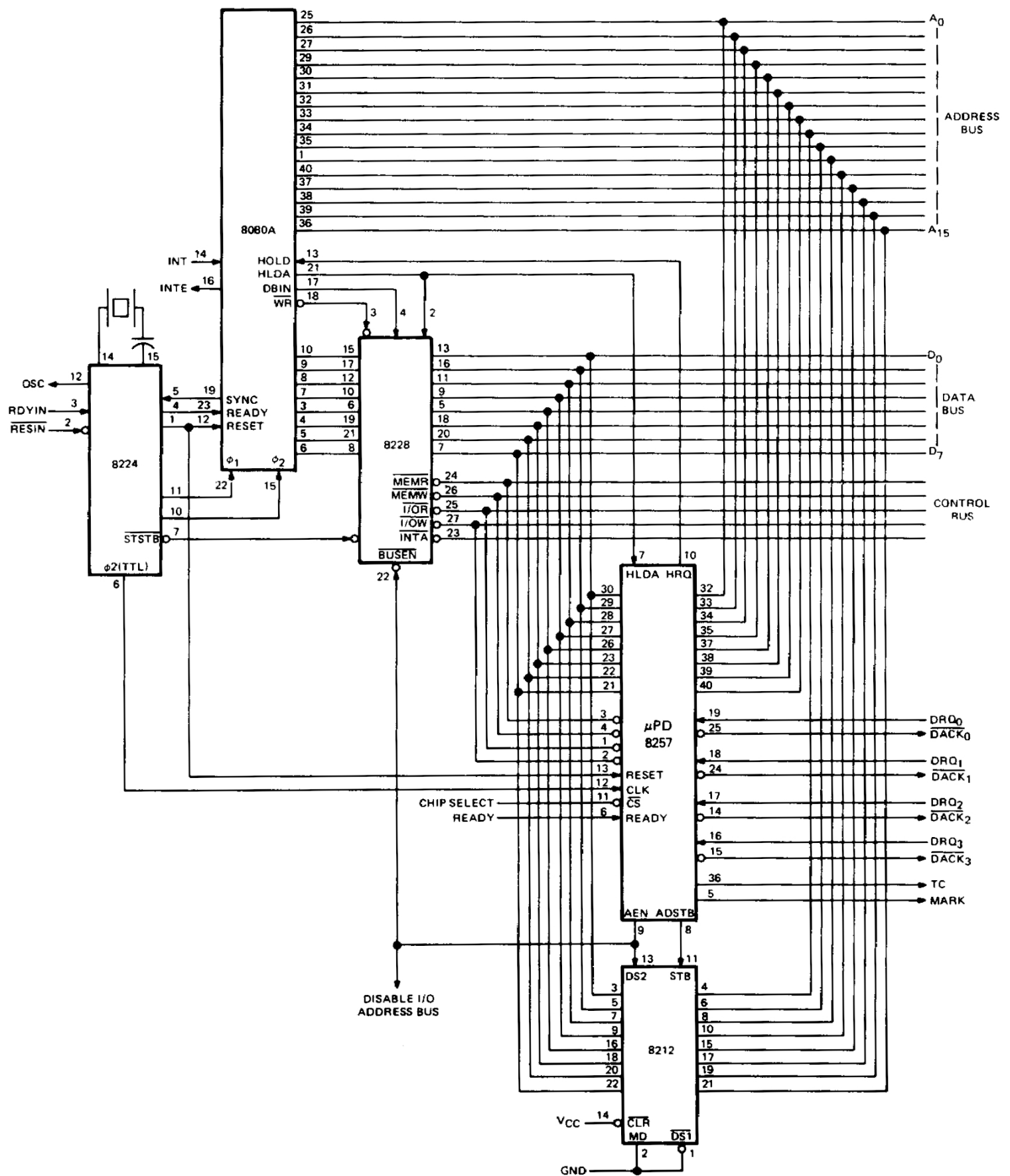
Figure 2. Typical \mu PD8257 System Interface Schematic
