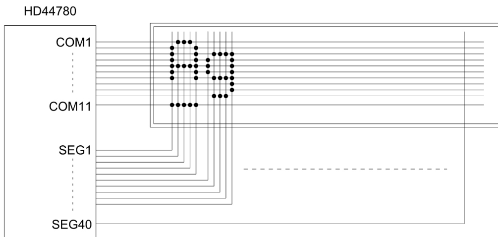
Example of a 5 \times 10 dot, 8-character \times 1-line display (1/4 bias, 1/11 duty cycle)
