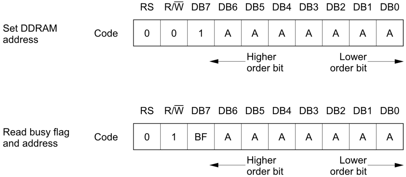
Figure 13 Instruction (2)
