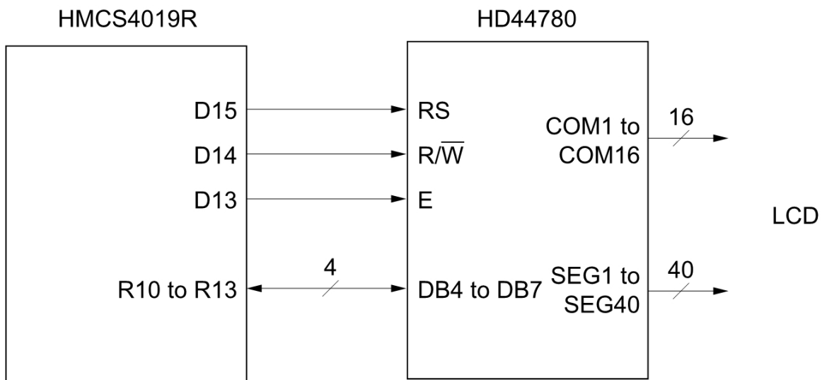
Figure 18 Example of Interface to HMCS4019R
