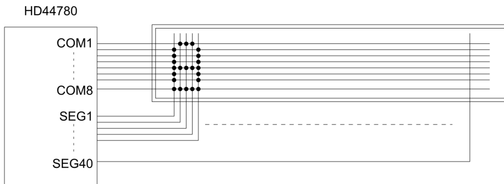
Example of a 5 \times 8 dot, 8-character \times 1-line display (1/4 bias, 1/8 duty cycle)
