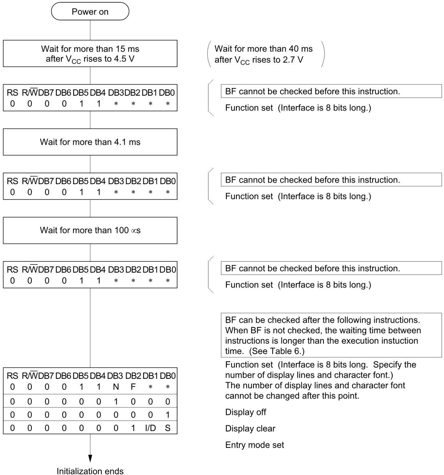
Figure 23 8-Bit Interface
