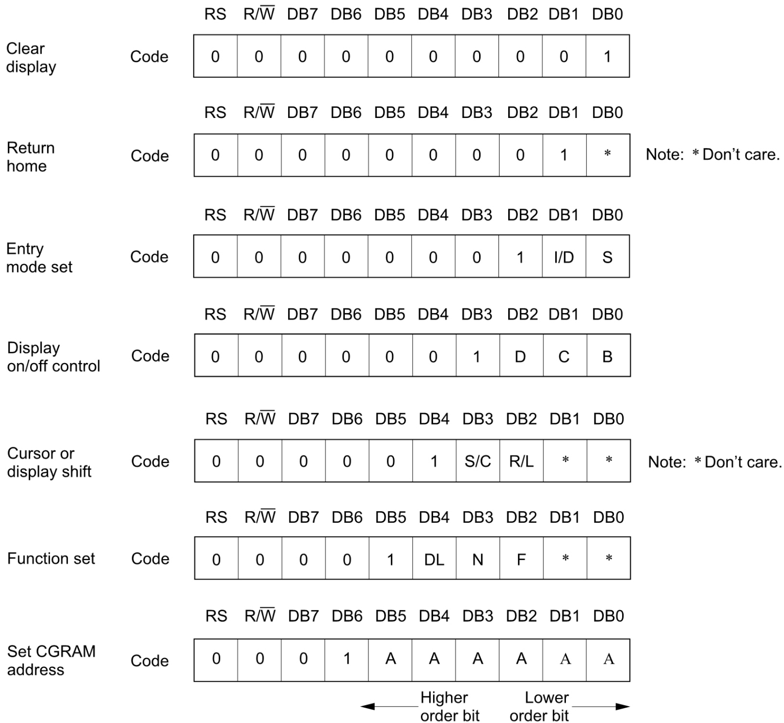
Figure 11 Instruction (1)
