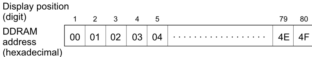
Figure 2 1-Line Display
