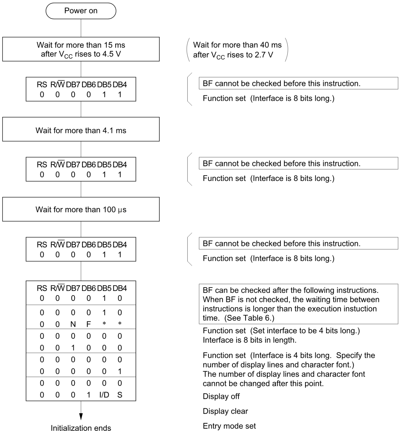
Figure 24 4-Bit Interface
