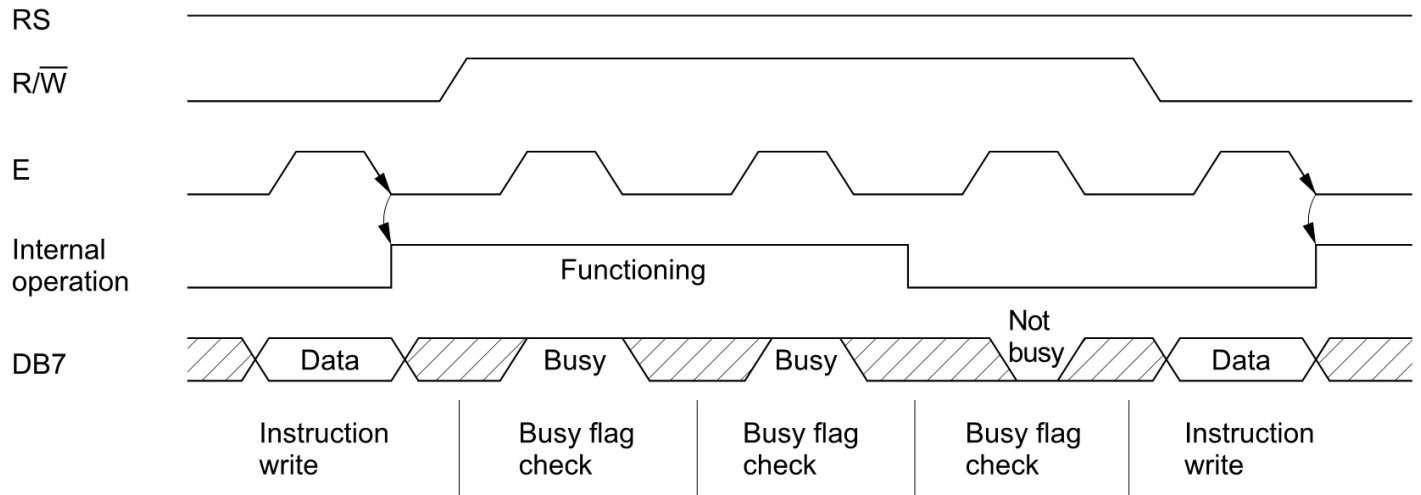
Figure 15 Example of Busy Flag Check Timing Sequence
