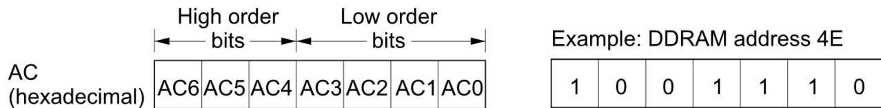
Figure 1 DDRAM Address
