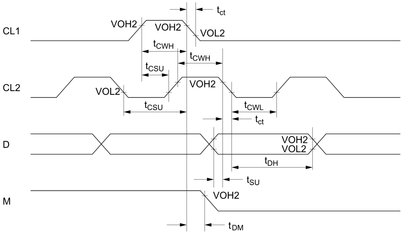
Figure 27 Interface Timing with External Driver
