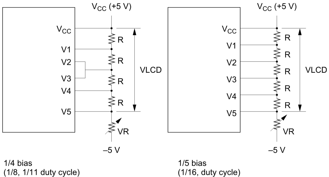
Figure 21 Drive Voltage Supply Example
