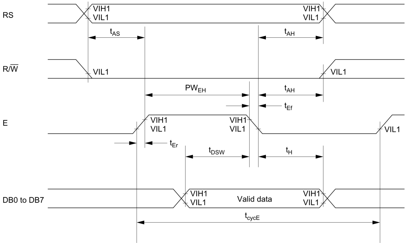
Figure 25 Write Operation
