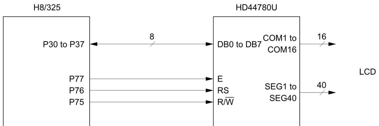
Figure 16 H8/325 Interface (Single-Chip Mode)
