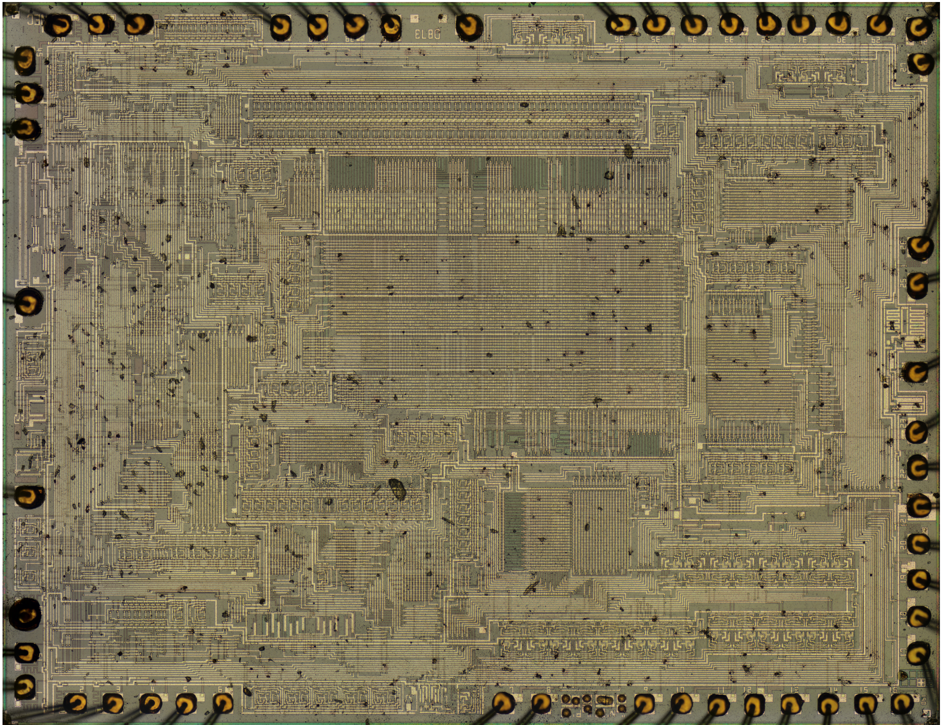
\mu PD873G 20x Die Photo 17000 x 13145 (224 MP) 6400% (64x) Tolerant Synthesized by Hugin
